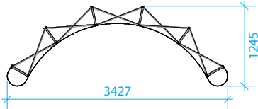
4x3 Curved Pop Up
